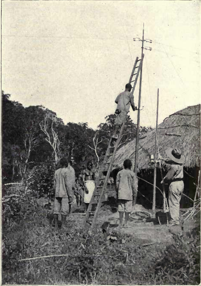
BRACKETING ON THE CAPE TO CAIRO TELEGRAPH.
